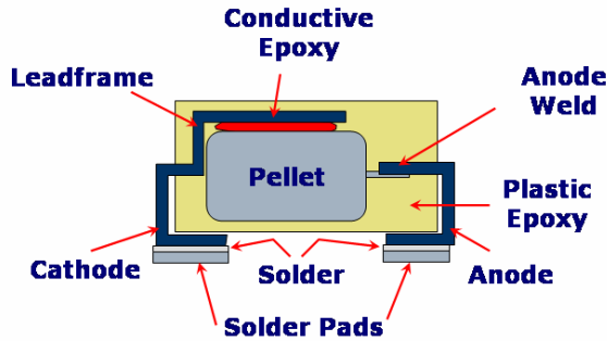
Figure 1. Standard surface-mount tantalum capacitor cutaway drawing.
