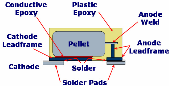
Figure 2. Cutaway view of facedown surface mount tantalum capacitor.
