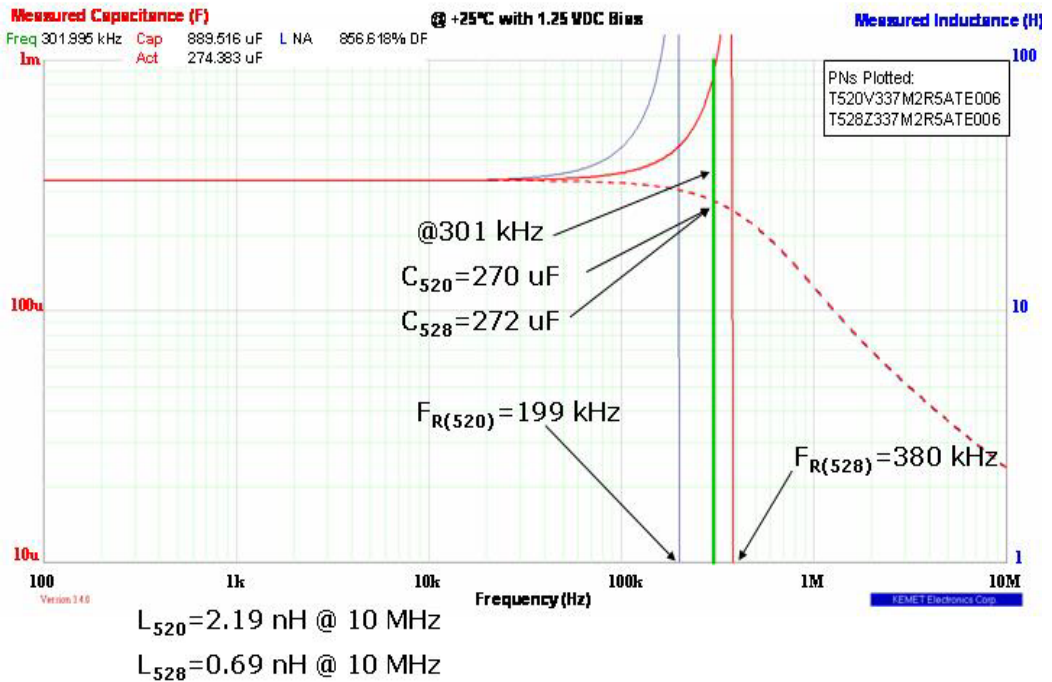
Figure 10. Capacitance versus frequency for the standard design (T520) and the facedown design (T528).
