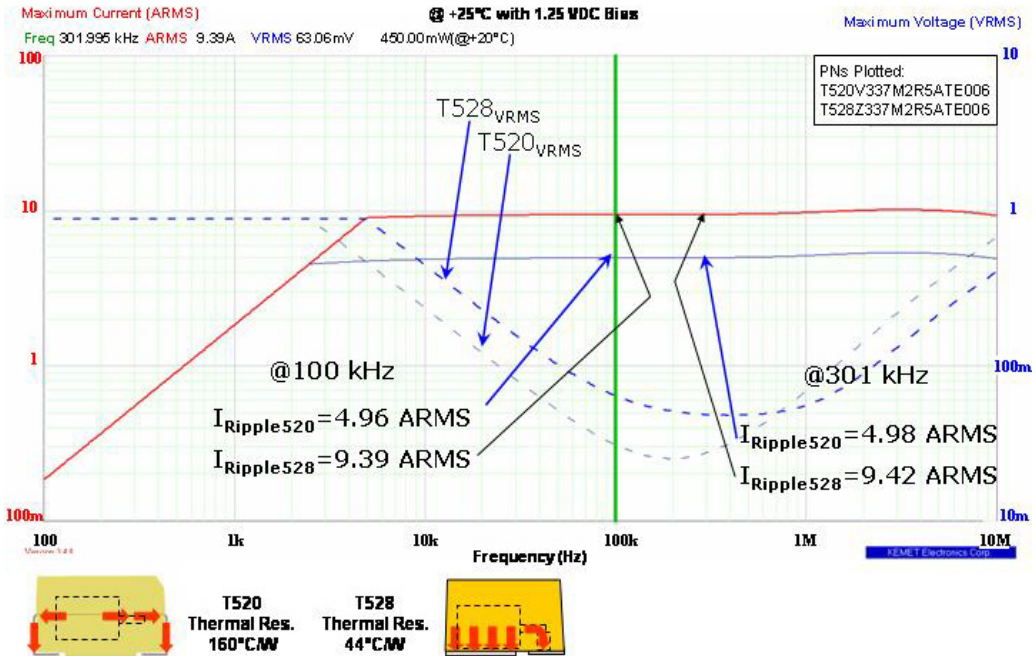
Figure 11. Ripple current versus frequency for the standard design versus the facedown design.
