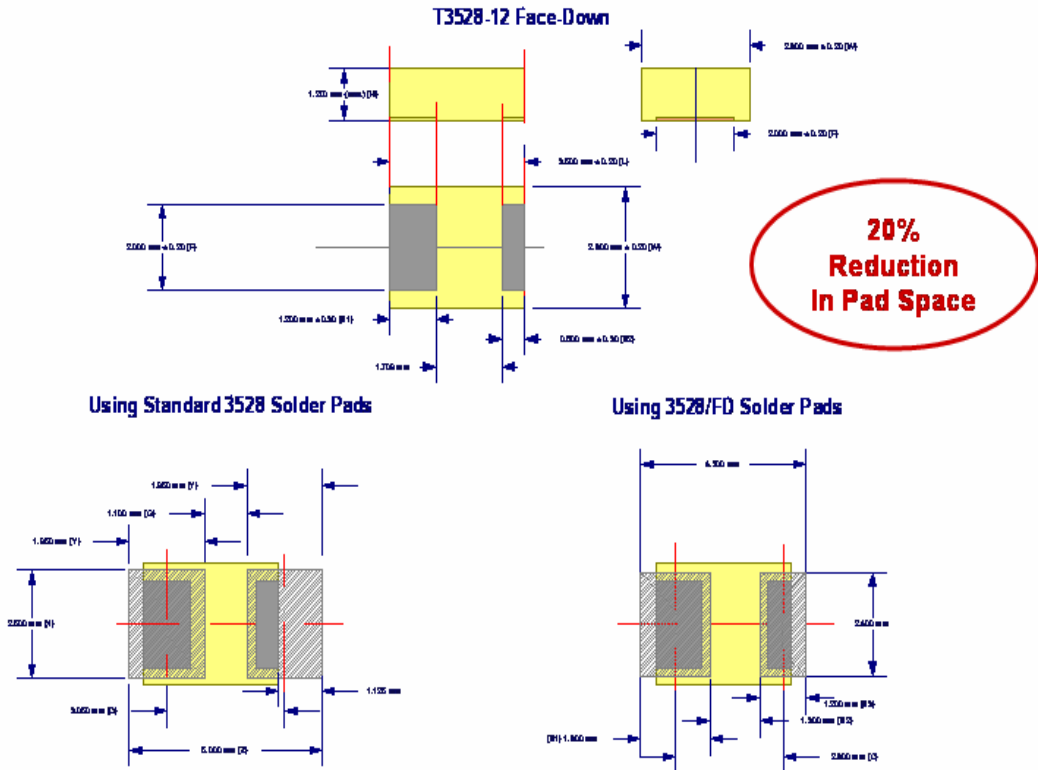
Figure 4. Solder pad dimensions and coverage for EIA 3528-12 case size.
