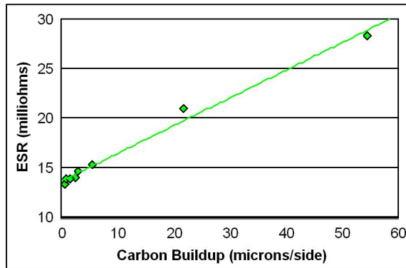
Figure 7. ESR versus carbon buildup.
