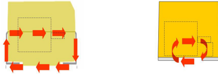
Figure 9. The decrease in current loop area with face down design compared to traditional surface mount device reduces ESL of the facedown configuration.
