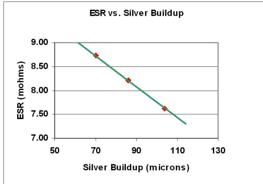
Figure 8. Relationship between ESR and silver buildup.
