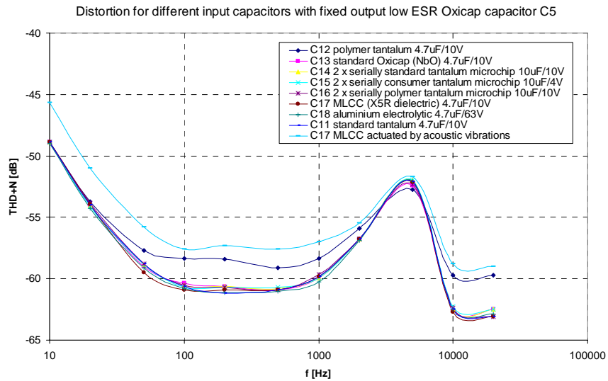
Figure 5: Harmonic distortion for different input coupling capacitors
