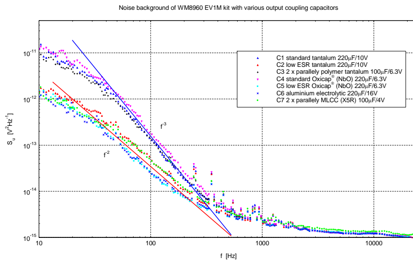
Figure 2: Results of background noise measurement
