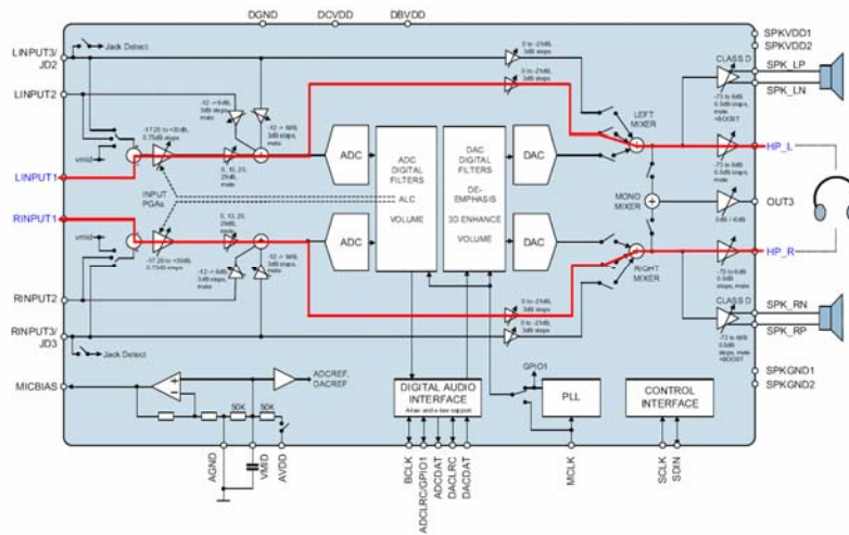
Figure 1: WM8960 codec internal configuration
