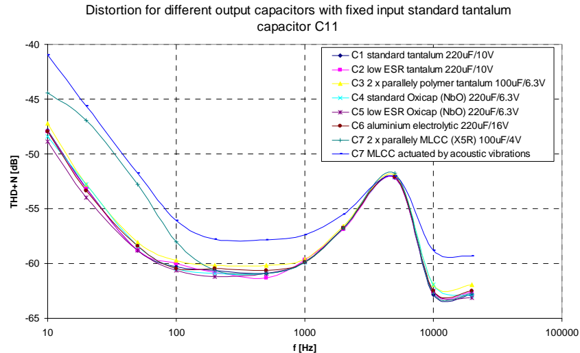
Figure 4: Harmonic distortion for different output coupling capacitors
